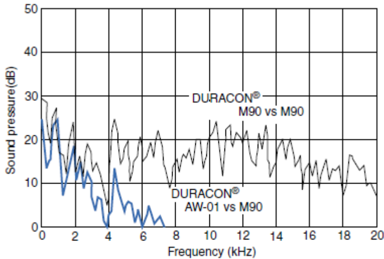
Fig.1-8 Frequency Analysis of Gear Noise, DURACON® POM vs. DURACON® POM(150rpm, 3.9×10 -2 N • m)
