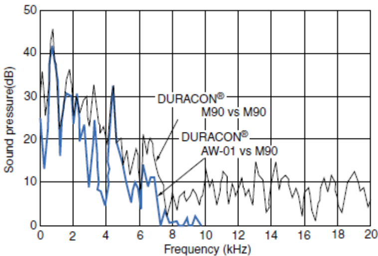
Fig.1-9 Frequency Analysis of Gear Noise, DURACON® POM vs. DURACON® POM(400rpm, 1.9×10 -2 N • m)
